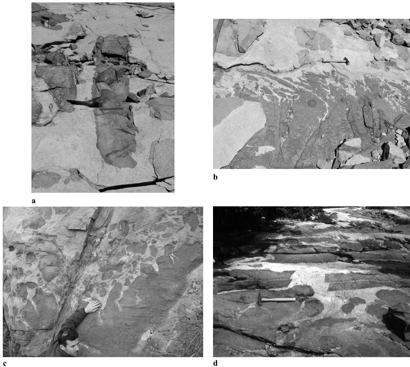
Fig. 1. Field photos showing characteristics of enclave formation. (a) Disrupted mafic dike with crenulate margin in the granitic Post Peak pluton, central Sierra Nevada, California. Dike width \sim 50 cm. (b) Close-up of another dike margin in the Post Peak pluton, showing disaggregation of dike and formation of enclaves. Note that some enclaves have large length/width ratios. Hammer for scale. (c) Margin of mafic dike in the Guadalupe Igneous Complex, Sierra Nevada, California, displaying disaggregation of dike and formation of enclaves. (d) Mafic sheets in Cadillac Mountain pluton, Maine showing disaggregation of sheets and formation of enclaves. See Wiebe (1994, 1996) for detailed discussion of this photo.
