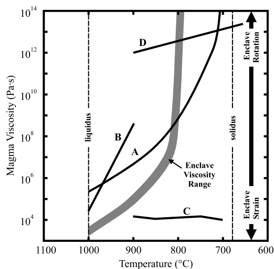
Fig. 3. Enclave viscosity plot combining data from different sources. Line A and 'Enclave Viscosity Range' are from Hrouda et al. (1999) for a granodiorite host. Line B is from Williams and Tobisch (1994) for a 65 wt% SiO 2 host. Line C is from Scaillet et al. (1998) for wet (3.5–7 wt% H 2 O) granite. Line D is from Rutter and Neumann (1995) for dry Westerly granite. Note the strong viscosity dependence on both temperature and H 2 O content.
